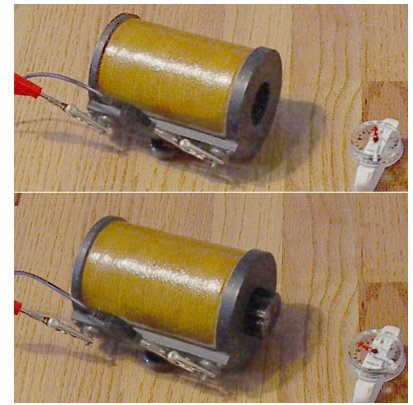
e / Example 24: without the iron core, the field is so weak that it barely deflects the compass. With it, the deflection is nearly 90^\circ .
